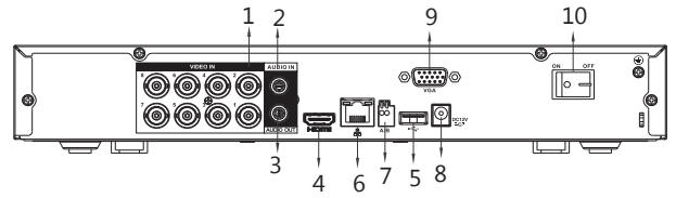
DH-XVR5108H-4KL-X
